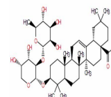
Chemical structure of A-Hederin
