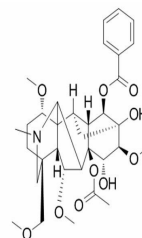
Chemical structure of Hypaconitine
