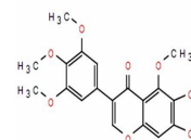
Chemical structure of Irisflorentin
