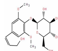
Chemical structure of Eleutheroside B
