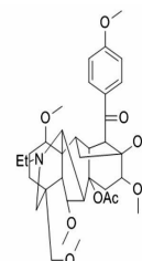
Chemical structure of Bulleyaconitine A
