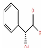
Chemical structure of Mandelic acid
