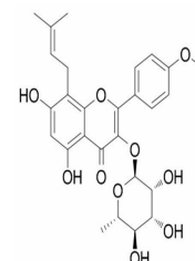
Chemical structure of baohuoside I
