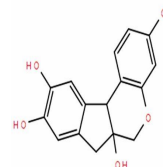
Chemical structure of Brazilin
