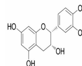
Chemical structure of L-Epicatechin
