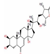
Chemical structure of Cyasterone
