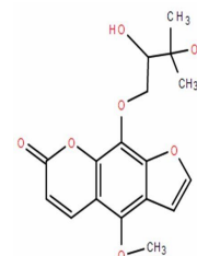
Chemical structure of Byakangelicin
