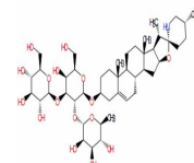
Chemical structure of Solasonine
