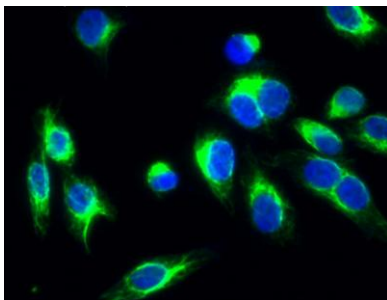
Immunofluorescence analysis of HeLa cell. 1,TPH1 Polyclonal Antibody(green) was diluted at 1:200(4° overnight). 2, Goat Anti Rabbit Alexa Fluor 488 Catalog:RS3211 was diluted at 1:1000(room temperature, 50min). 3 DAPI(blue) 10min.
