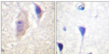
Immunohistochemistry analysis of paraffin-embedded human brain, using Bcr (Phospho-Tyr360) Antibody. The picture on the right is blocked with the phospho peptide.
