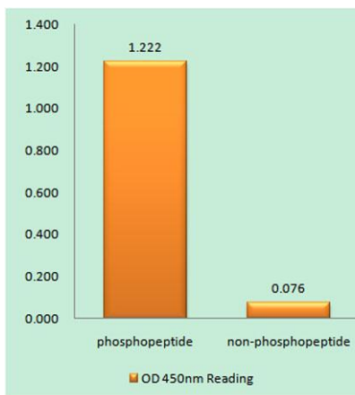
Enzyme-Linked Immunosorbent Assay (Phospho-ELISA) for Immunogen Phosphopeptide (Phospho-left) and Non-Phosphopeptide (Phospho-right), using Bcr (Phospho-Tyr360) Antibody
