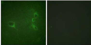
Immunofluorescence analysis of NIH/3T3 cells, using Bcr (Phospho-Tyr360) Antibody. The picture on the right is blocked with the phospho peptide.
