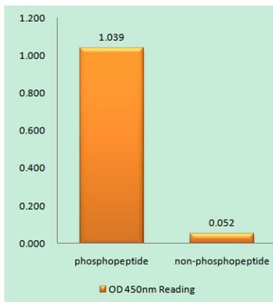
Enzyme-Linked Immunosorbent Assay (Phospho-ELISA) for Immunogen Phosphopeptide (Phospho-left) and Non-Phosphopeptide (Phospho-right), using FAK (Phospho-Tyr925) Antibody
