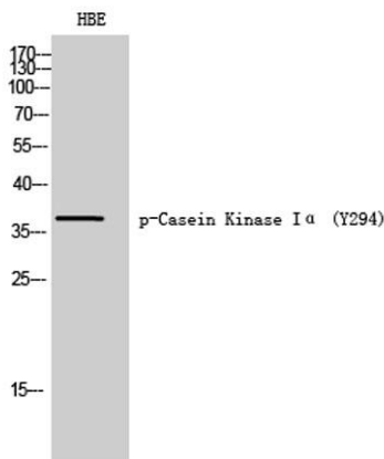
Western Blot analysis of HBE cells using Phospho-Casein Kinase Iα (Y294) Polyclonal Antibody diluted at 1:1000
