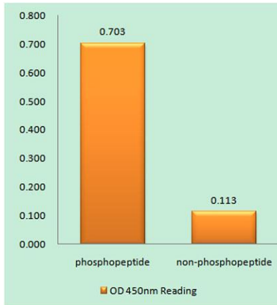
Enzyme-Linked Immunosorbent Assay (Phospho-ELISA) for Immunogen Phosphopeptide (Phospho-left) and Non-Phosphopeptide (Phospho-right), using CK-1 alpha (Phospho-Tyr294) Antibody
