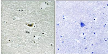
Immunohistochemistry analysis of paraffin-embedded human brain, using CK-1 alpha (Phospho-Tyr294) Antibody. The picture on the right is blocked with the phosphopeptide.
