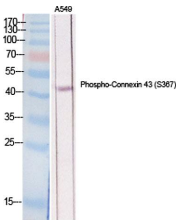
Western Blot analysis of various cells using Phospho-Connexin 43 (S367) Polyclonal Antibody diluted at 1:2000
