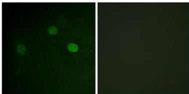
Immunofluorescence analysis of COS7 cells, using CDK1/CDC2 (Phospho-Thr14) Antibody. The picture on the right is blocked with the phospho peptide.
