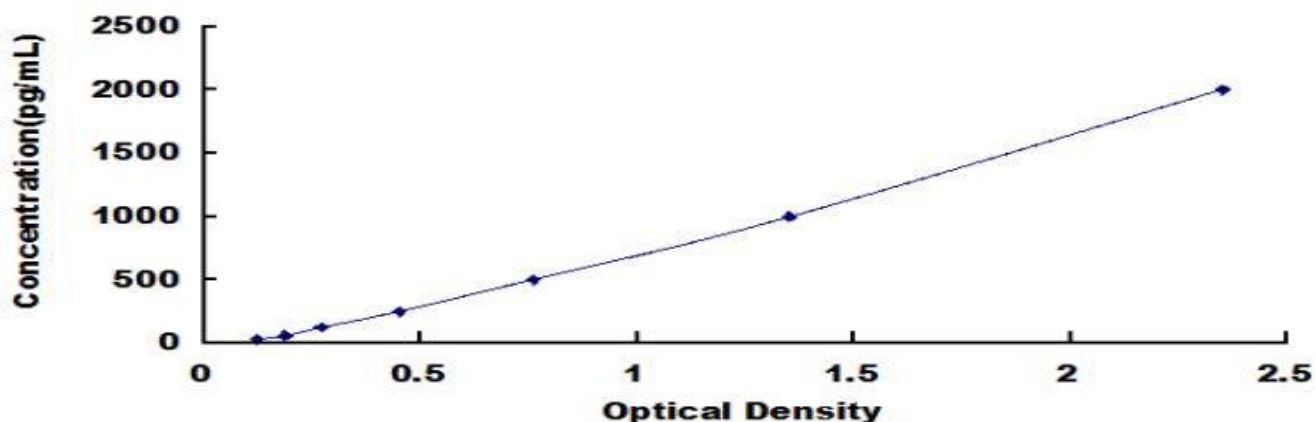
Typical Standard Curve for Mouse TGFb2 ELISA.
